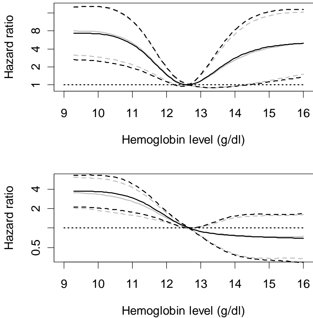
Fig. 5: Adjusted hazard ratio for ESA users (top) and non-users (bottom) at various hemoglobin levels vs. a reference level of 12.5 g/dl. Gray: original analysis (multiple imputation; N=1794, 286 events), black: analysis after multiple imputation of artificially generated nonrandomly missing data
