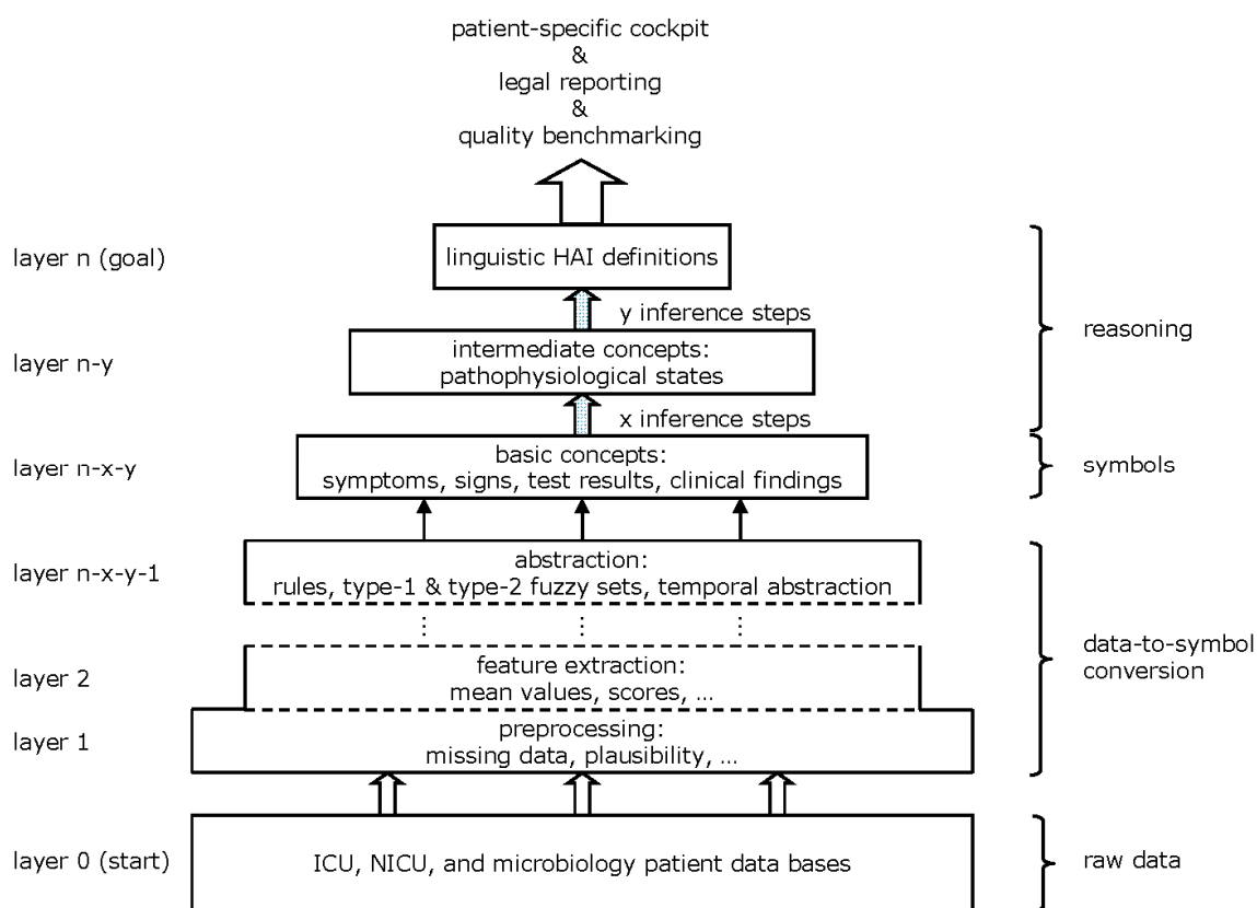
Figure 1: Data processing layers in MONI explaining the way from raw data input [of electronic bedside sensors (e.g., pulse, blood pressure, body temperature), from biochemical laboratory (e.g., leucocyte count, erythrocyte sedimentation rate, C-reactive protein), from microbiology and from routine bedside data entries by ICU staff] to the required specific outputs. HAI: healthcare associated infection, ICU: intensive care unit, NICU: neonatal intensive care unit.
