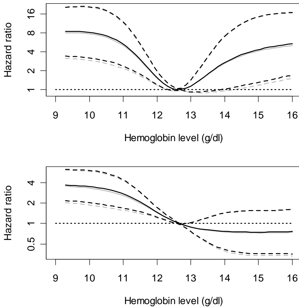
Fig. 13: Adjusted hazard ratio for ESA users (top) and non-users (bottom) at various hemoglobin levels vs. a reference level of 12.5 g/dl. Gray: original analysis (multiple imputation; N=1794, 286 events, follow-up until 31 Dec 2004), black: analysis excluding cardiovascular disease variables from final model.
